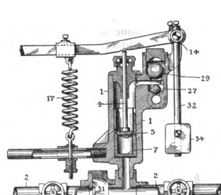
WASHBURNE FUEL FEED DEVICE.
